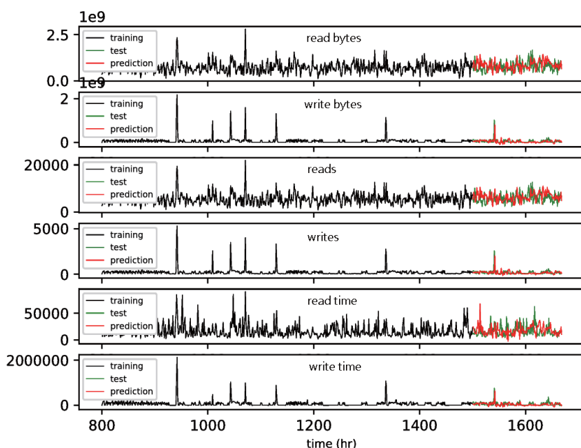
Figure 1: Disk I/O Performance Prediction by LSTM
